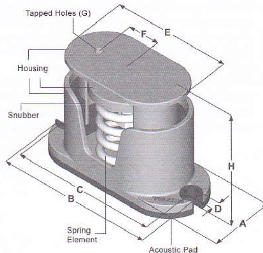
PTM-CH, PTM-CH2
