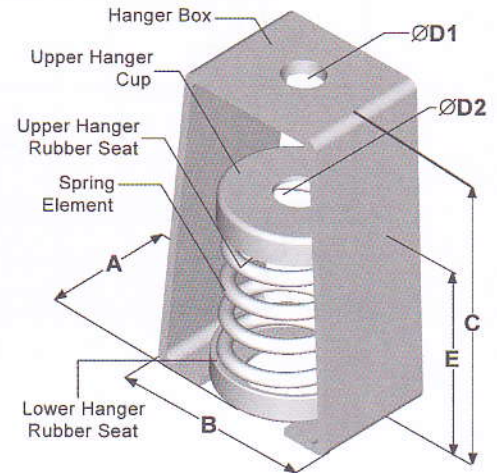
PTH-S-xxx,M PTH-S2-xxxS
