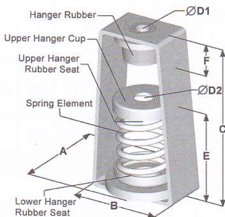
PTH-SG-xxxM, PTH-SG2-xxxM
