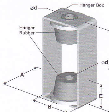
PTH-GG-80, 120, 150, 200, 300, 450
