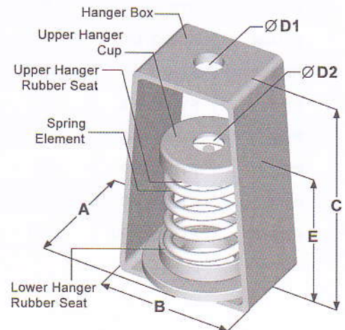
PTH-S-xxxxM PTH-S2-xxxxM
