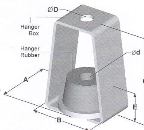
PTH-G-80, 120, 150, 200, 300, 450
