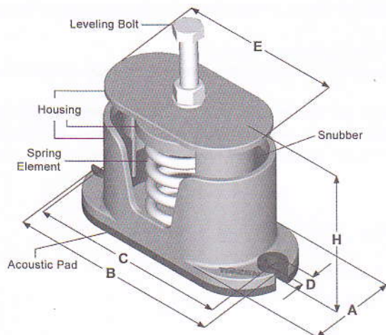
PTM-C, PTM-C2
