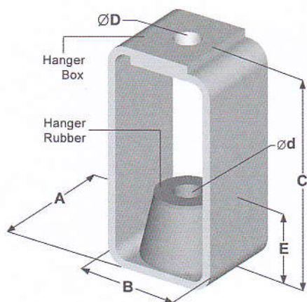
PTH-G-25, 35, 50
