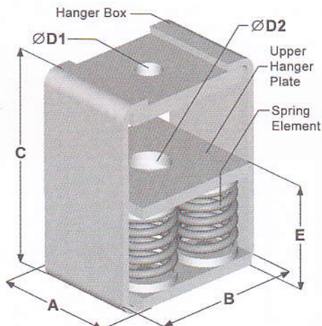
PTH-S-xxx4M, PTH-S2-xxx4M
